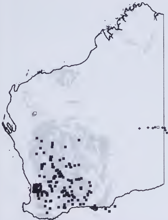
Figure 7. Distribution of three Ctenophorus dragon lizards ( C. ornatus ■; C. rufescens □; C. yinnietharra □) and a gecko ( Gehyra montium +) with respect to granite landforms (dark gray shading) in Western Australia (modified from Withers & Edward 1977). Locality data from Western Australian Museum.
